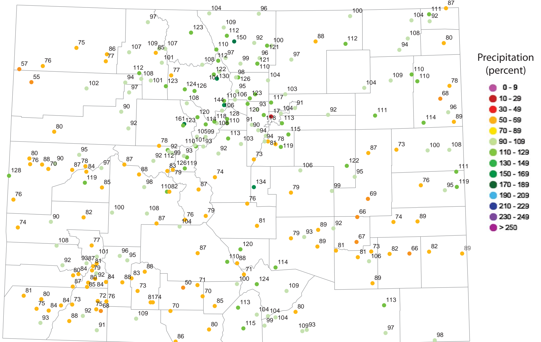
Water Year 2003 (October 2002 through September 2003) precipitation as a percent of the 1971-2000 average.
