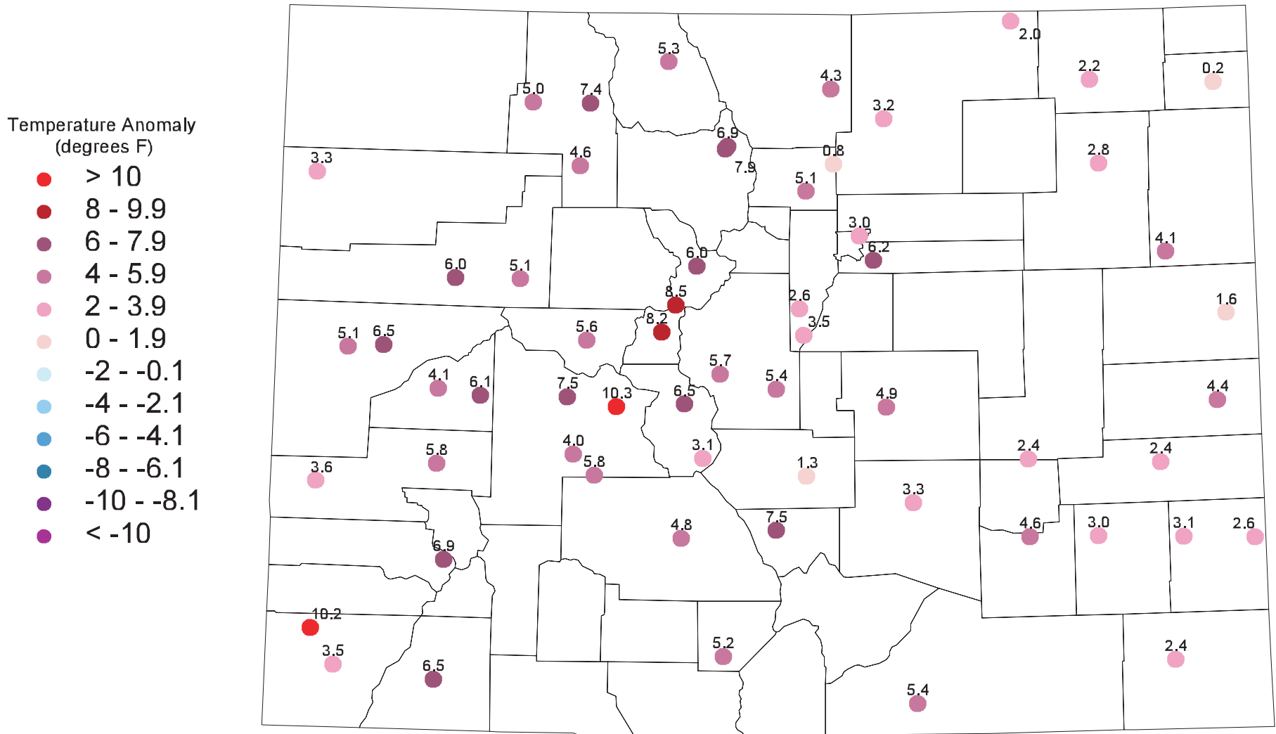
April 2002 temperature departures from the 1961-90 average.
