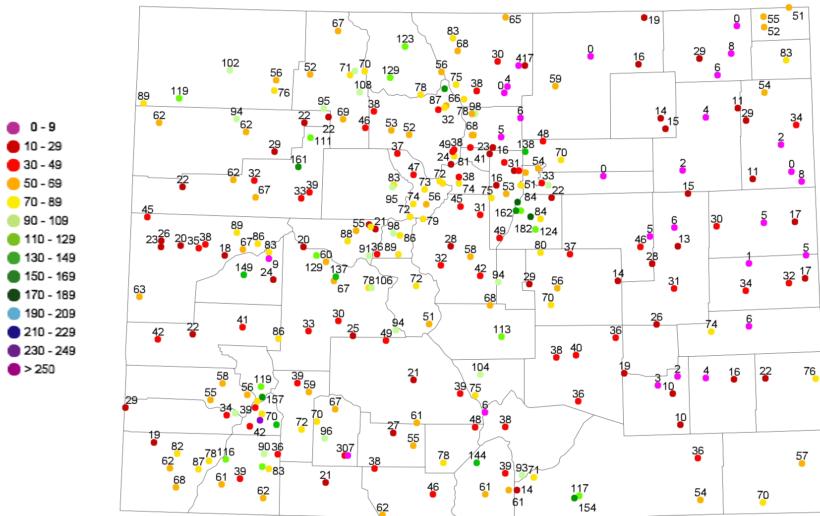
July 2002 precipitation percent of 1961-1990 average.
