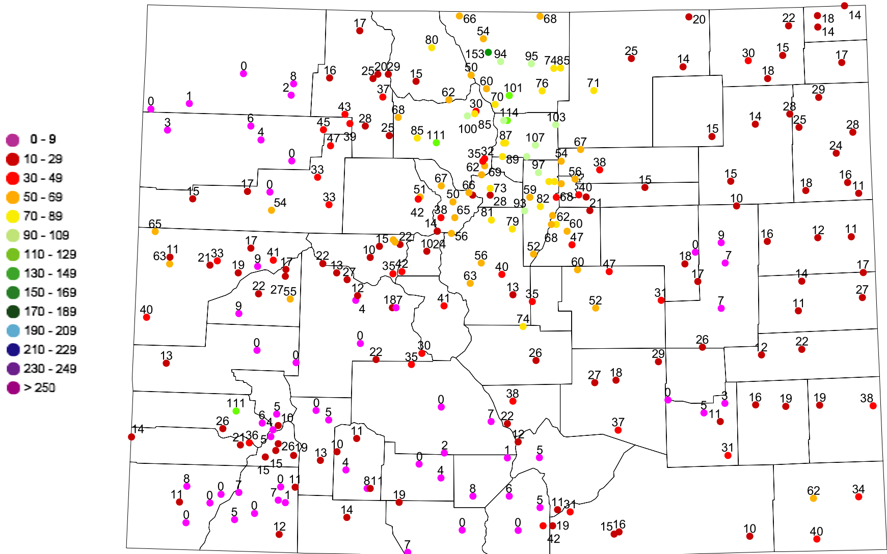
May 2002 precipitation as a percent of the 1961-1990 average.
