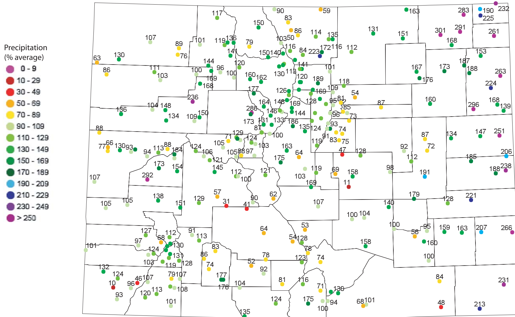
October 2002 precipitation as a percent of average for the 1961-1990 average.
