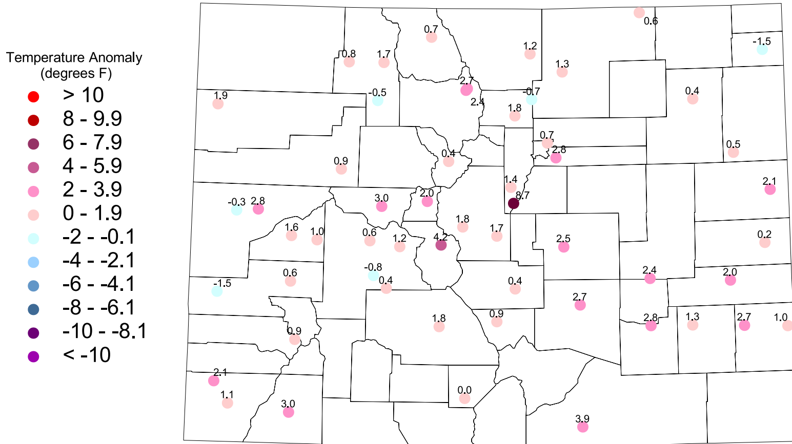
August 2002 temperature departures from the 1961-1990 average.
