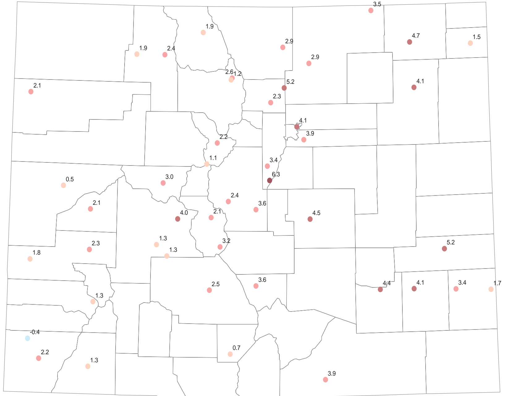
April 2003 temperature departures from the 1971-2000 averages.
