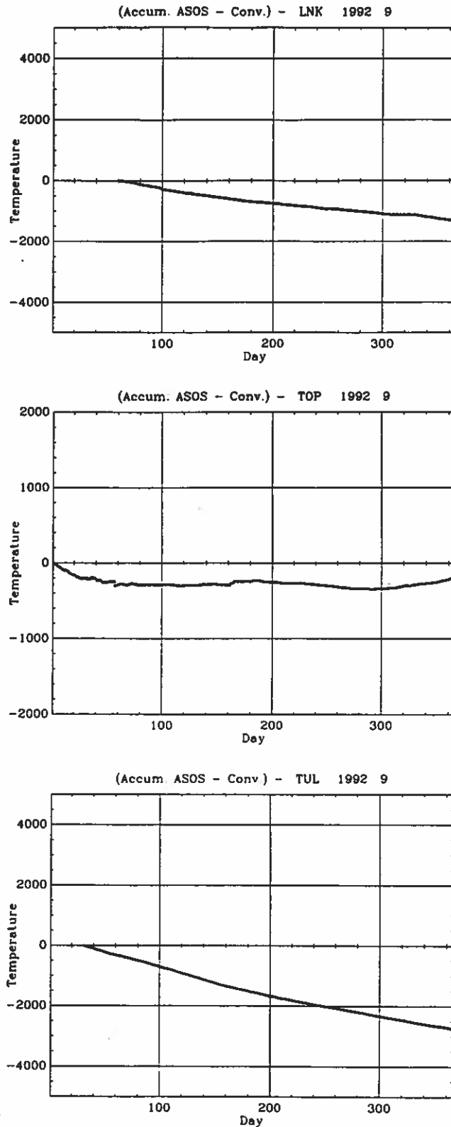
Figure 8. ASOS - CONV accumulated temperature differences for LNK, TOP, and TUL. Data are based on observations at six-hour intervals from date of commissioning through August 1993. Note: different scaling is used for LNK and TUL due to larger temperature differences at those sites.
