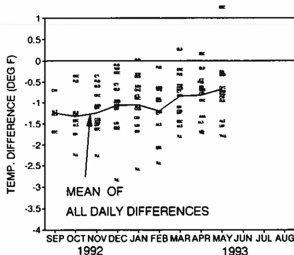
Figure 2. ASOS-CONV maximum temperature differences – commissioned sites only.
