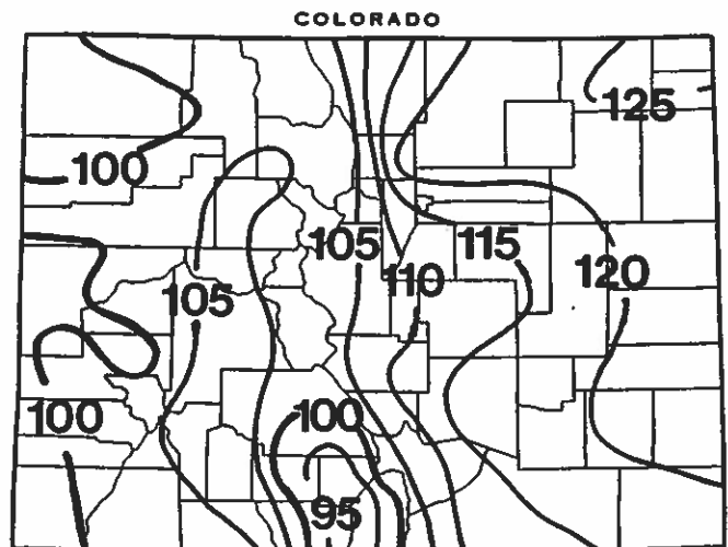
Accumulated Heating Degree Days for November 1992-March 1993 as a percent of November 1991-March 1992.
