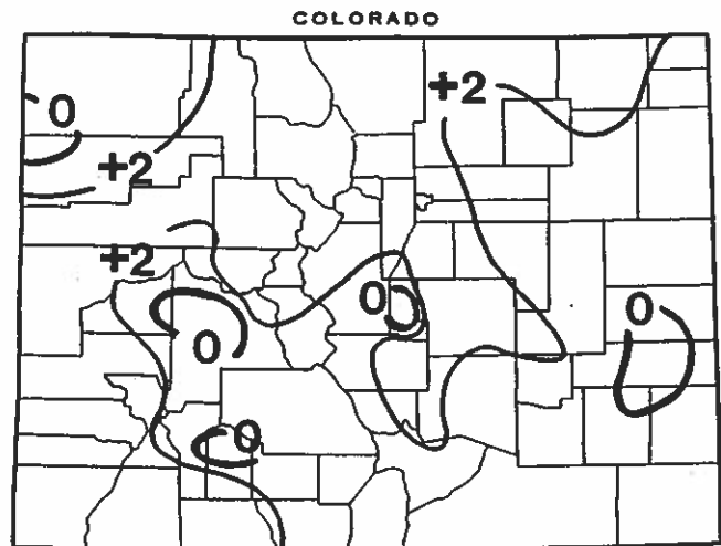
Departure of March 1993 temperatures from the 1961-90 averages.
