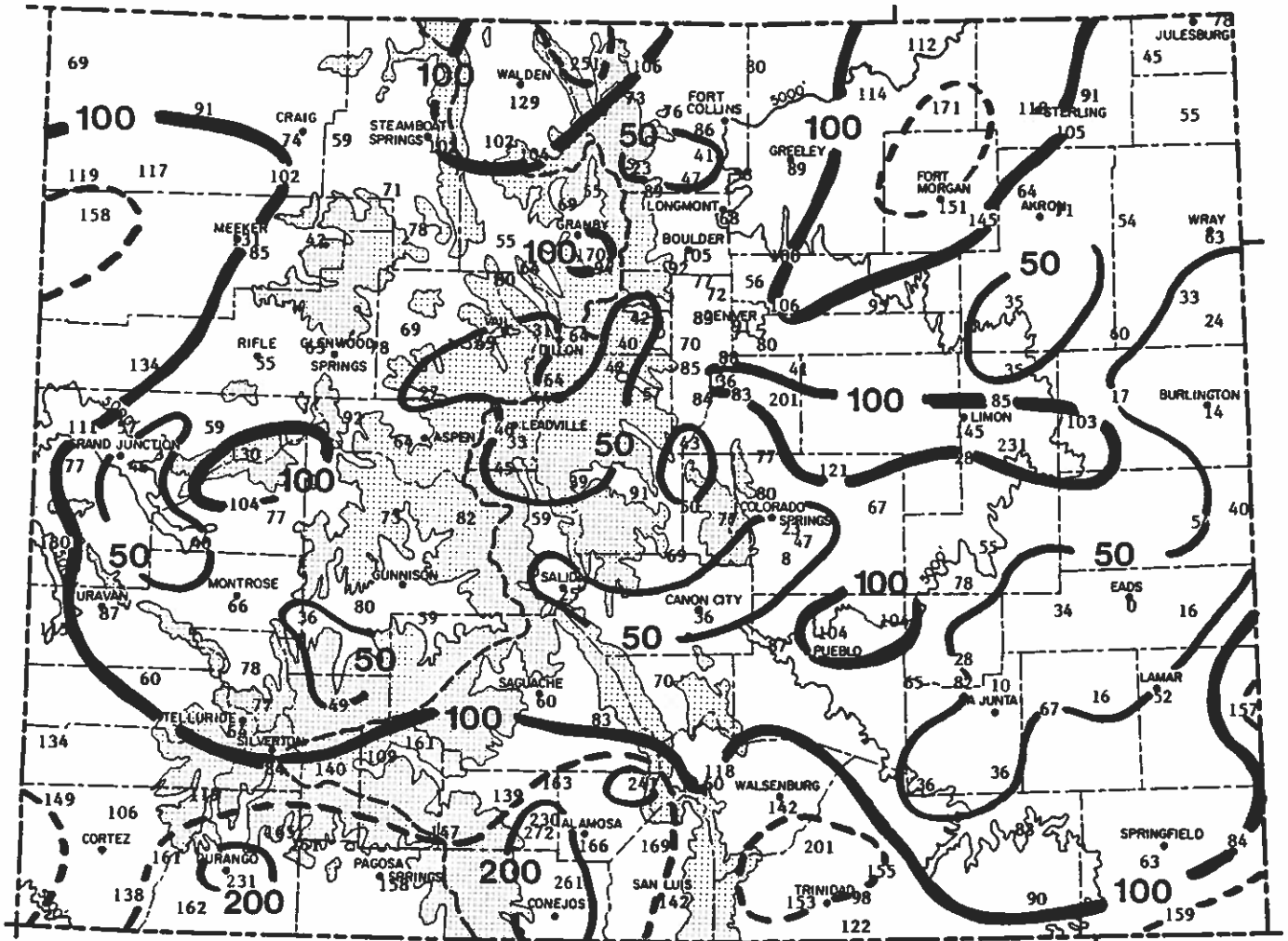
December 1992 Precipitation as a Percent of the 1961-90 average.
