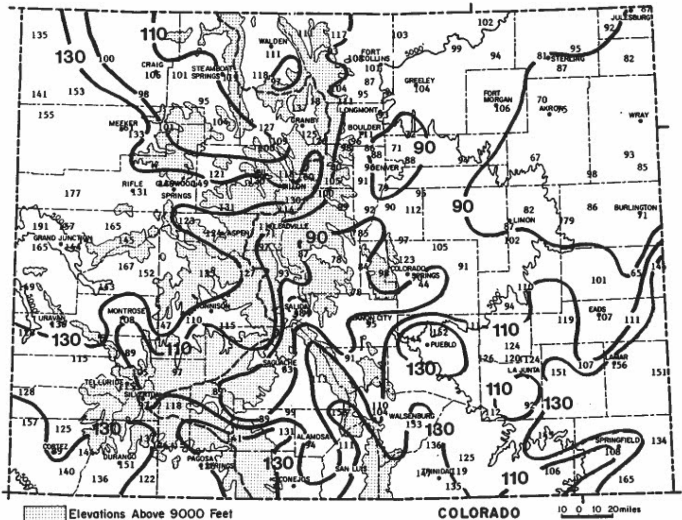
October 1992–June 1993 Precipitation as a Percent of the 1961-90 averages.
