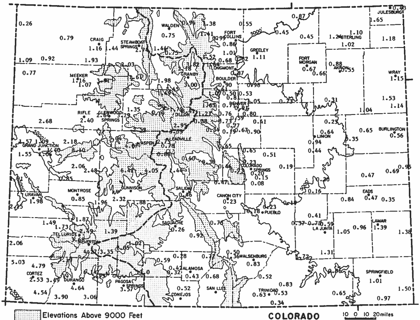
Precipitation Amounts (in inches) for February 1993.
