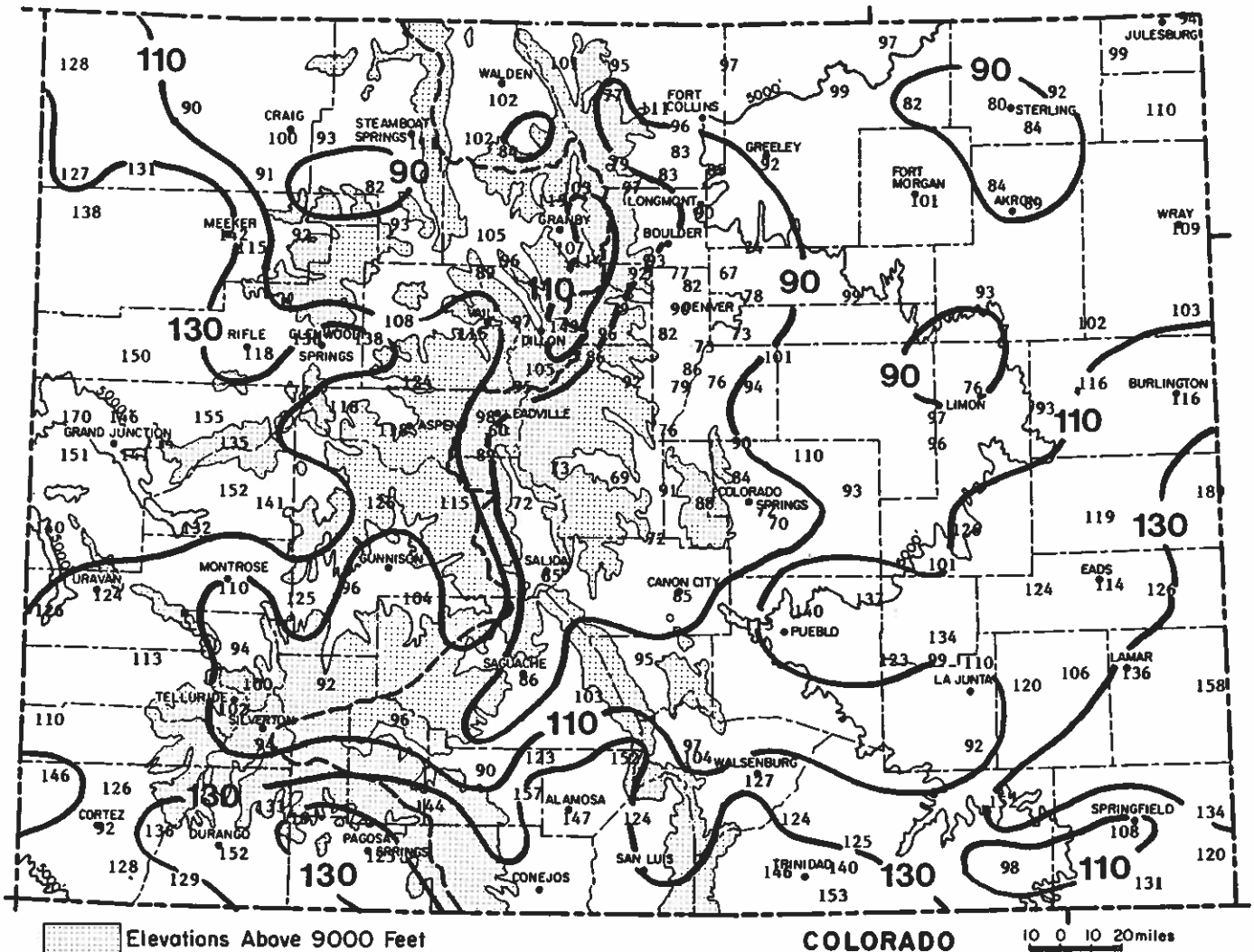
October 1992–August 1993 Precipitation as a Percent of the 1961-90 averages.
