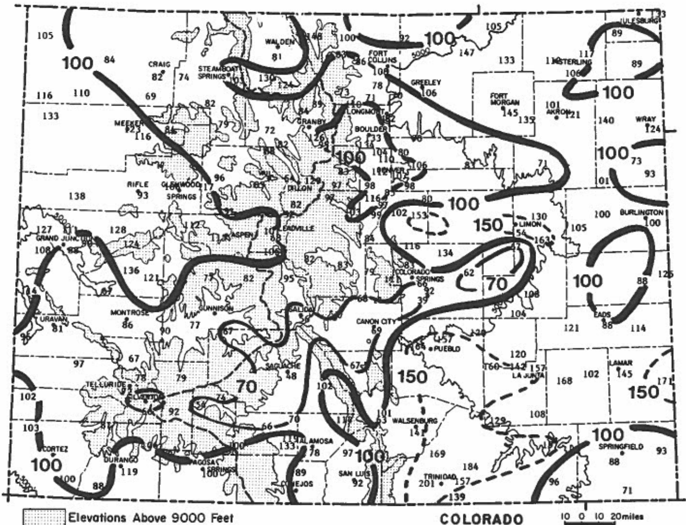
October-December 1992 Precipitation as a Percent of the 1961-90 averages.
