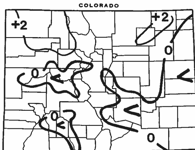
Departure of May 1993 temperatures from the 1961-90 averages.
