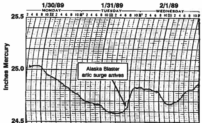
Fort Collins Station Pressure.
