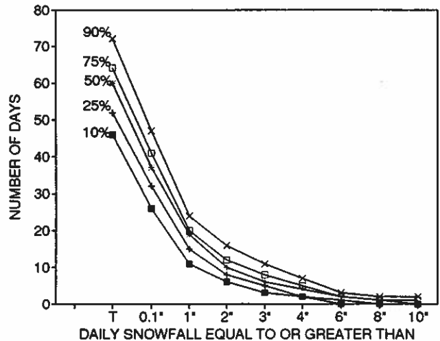
NONEXCEEDANCE PROBABILITY CURVES DENVER, COLORADO
