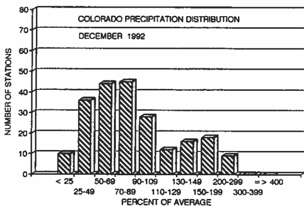
December 1992 Precipitation as a Percent of the 1961-90 average.
