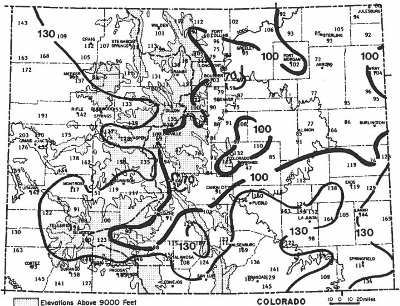
October 1992–May 1993 Precipitation as a Percent of the 1961-90 averages.
