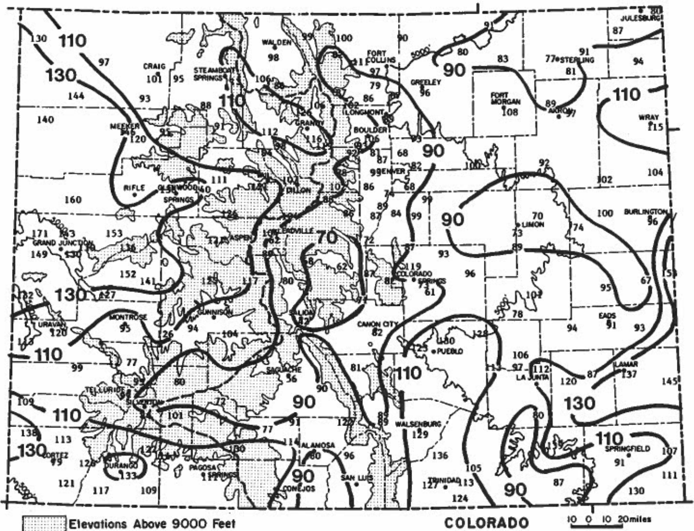
October 1992–July 1993 Precipitation as a Percent of the 1961-90 averages.
