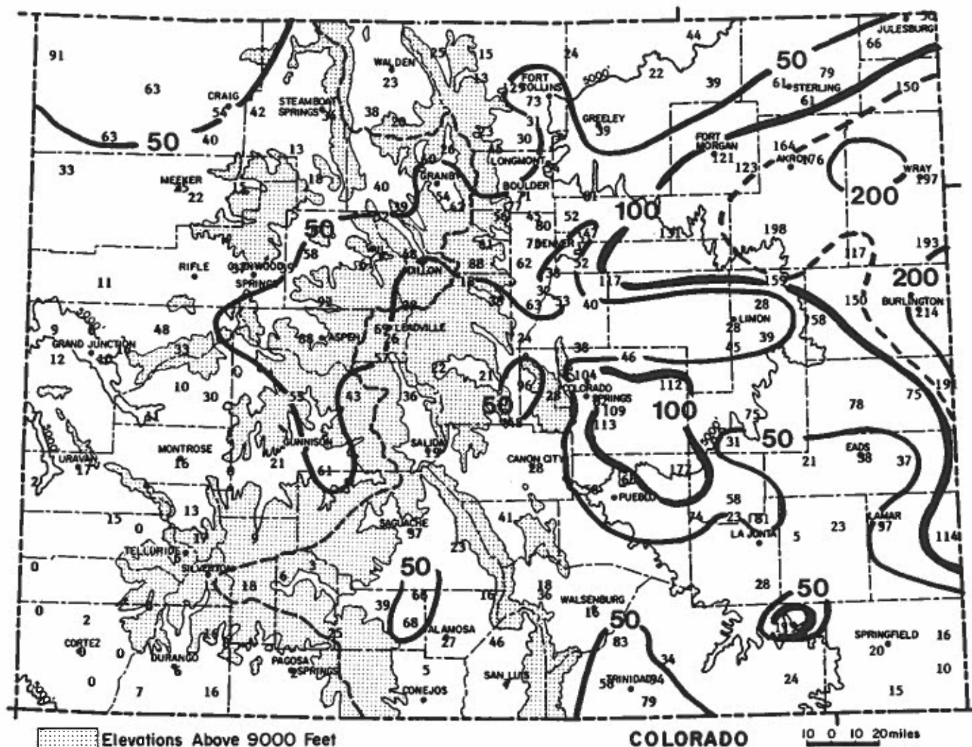
July 1993 Precipitation as a Percent of the 1961-90 average.
