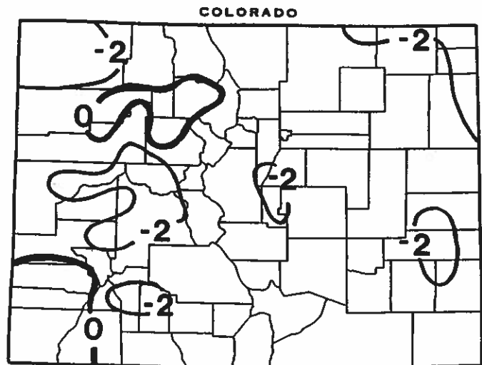
Departure of April 1993 temperatures from the 1961-90 averages.
