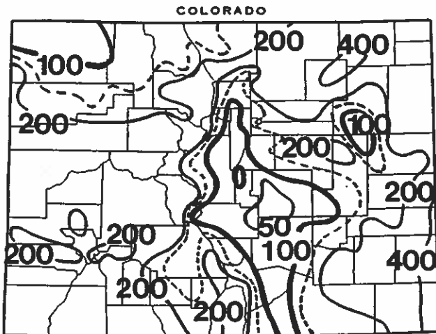
February 1993 precipitation as a percent of the 1961-1990 average. In extreme southwestern Colorado, where 3 to 4 times the average precipitation fell, this was one of the wettest February's on record. Much of eastern Colorado
