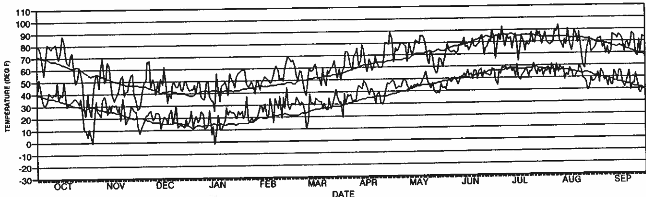
DAILY TEMPERATURES -- 1992 WATER YEAR FORT COLLINS, COLORADO
