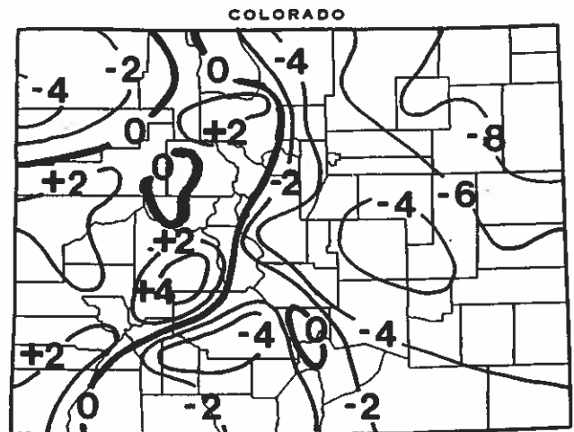
Departure of February 1993 temperatures from the 1961-90 averages.
