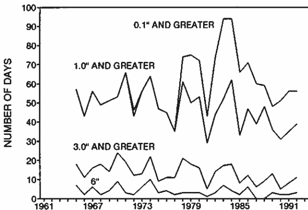
ANNUAL VARIATION IN NUMBER OF SNOW DAYS DILLON, COLORADO
