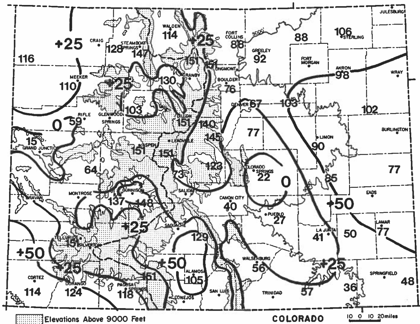
Number of days, November 1992–March 1993, with \geq 1 " snow on the ground and contours of departures from the 1961-1990 average.
