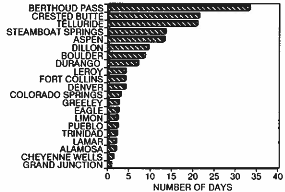
AVERAGE NUMBER OF DAYS WITH DAILY SNOWFALL OF EIGHT INCHES OR MORE
