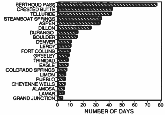
AVERAGE NUMBER OF DAYS WITH DAILY SNOWFALL OF FOUR INCHES OR MORE
