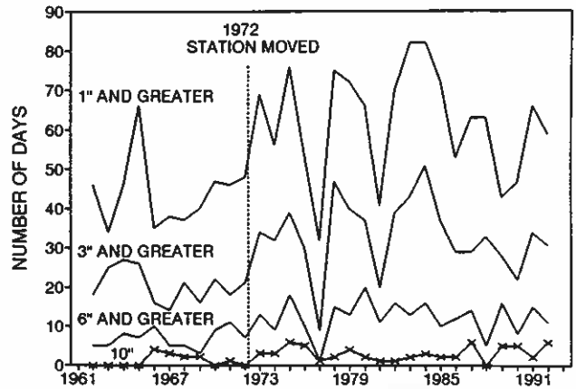
ANNUAL VARIATION IN NUMBER OF SNOW DAYS TELLURIDE, COLORADO
