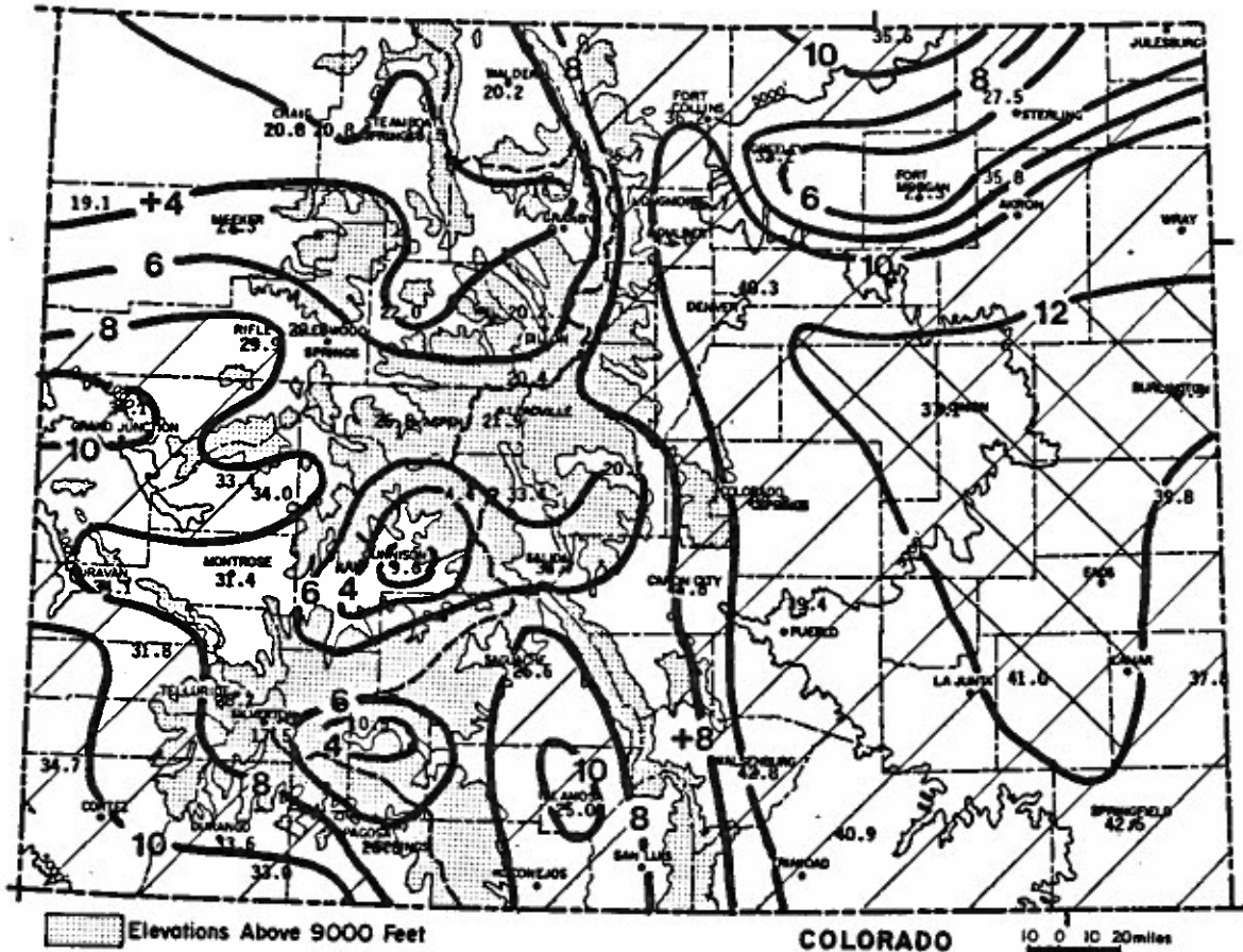
January 1986 temperatures (degrees Fahrenheit) and contours of departures from 1961-1980 averages.
