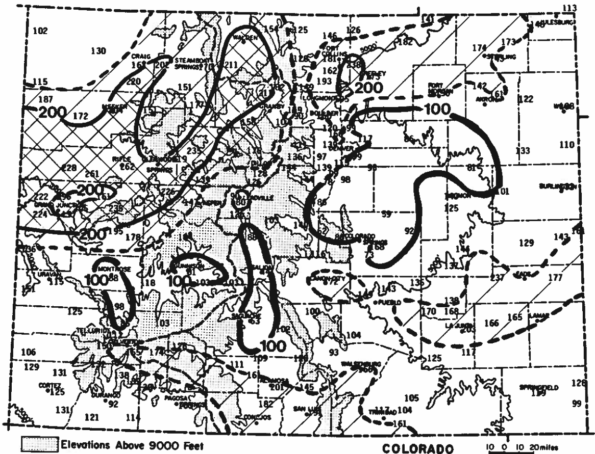
Precipitation for October 1985 through December 1985 as a percent of the 1961-1980 average. Dashed lines represent 150% of average.
