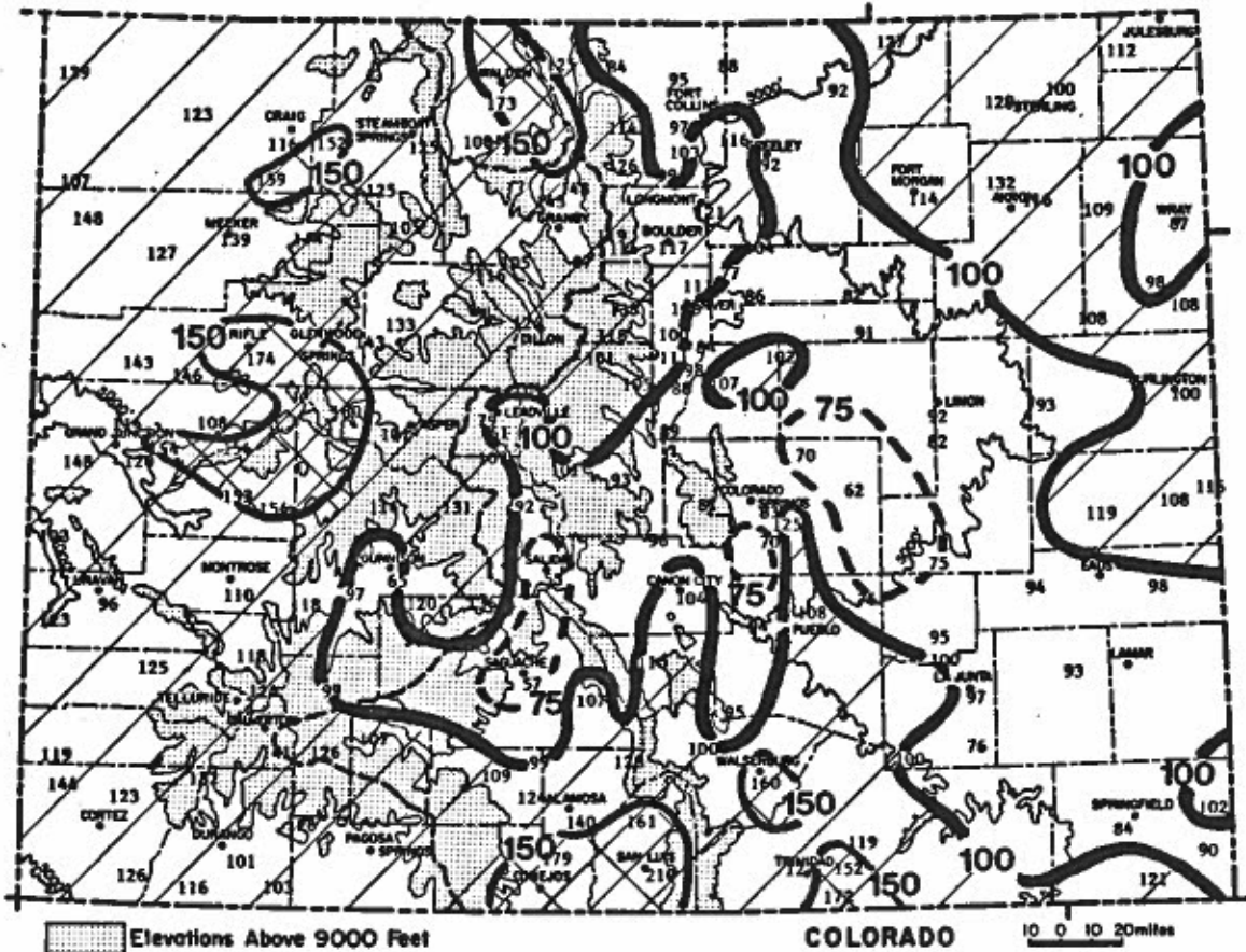
Precipitation for October 1985 through June 1986 as a percent of the 1961-1980 average.
