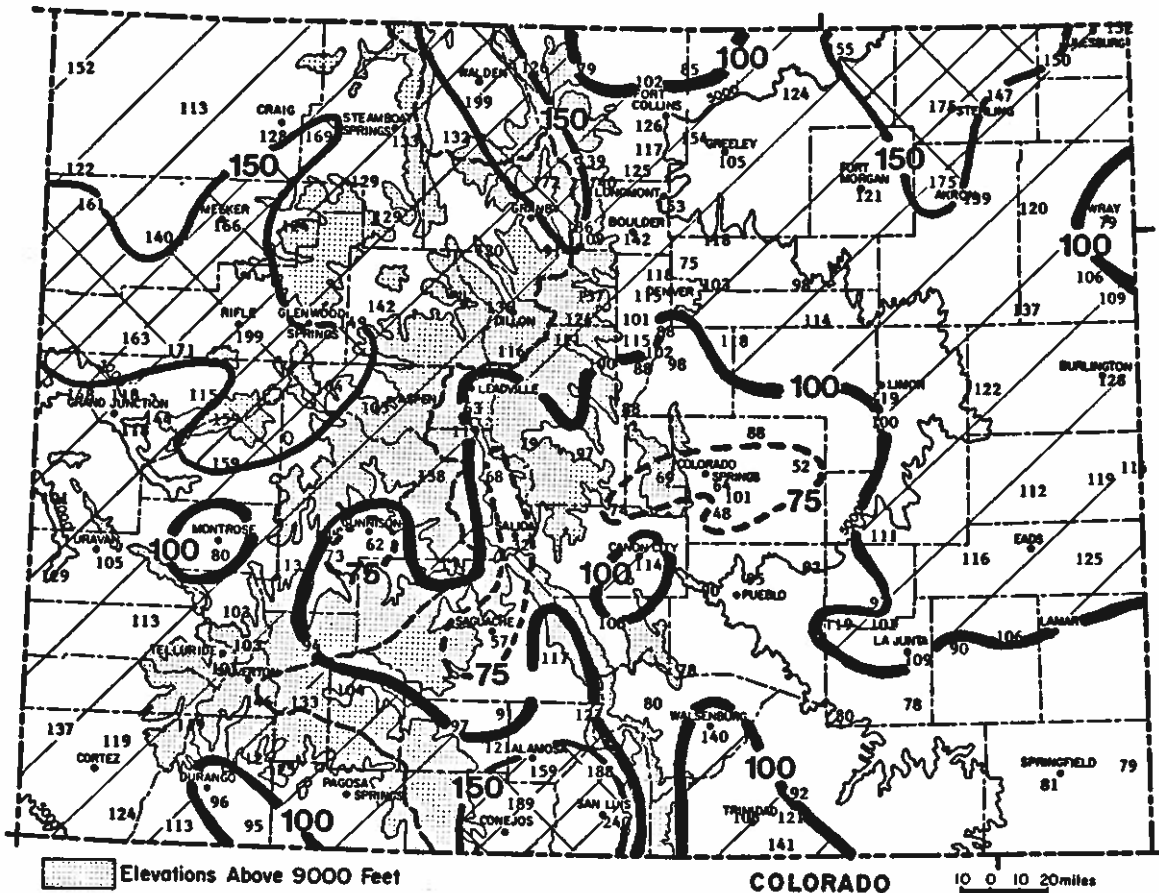
Precipitation for October 1985 through April 1986 as a percent of the 1961-1980 average.
