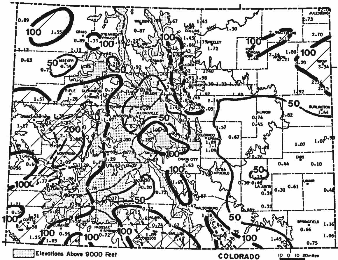
Precipitation amounts (inches) for May 1986 and contours of precipitation as a percent of the 1961-1980 average. The dashed line represents 150% of average.
