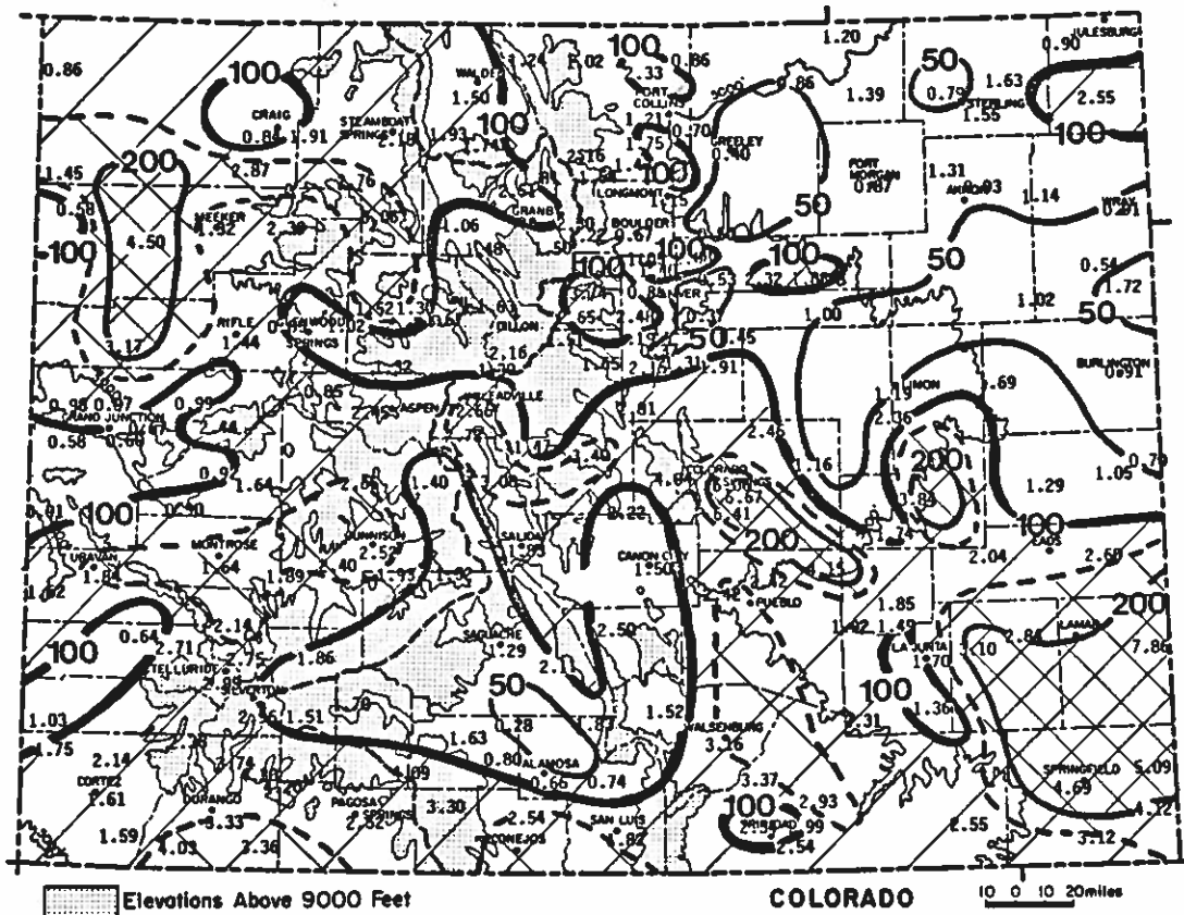
Precipitation amounts (inches) for August 1986 and contours of precipitation as a percent of the 1961-1980 average. The dashed line represents 150% of average.
