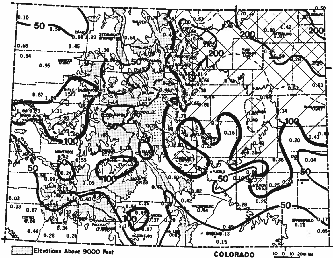
Precipitation amounts (inches) for December 1985 and contours of precipitation as a percent of the 1961-1980 average. Dashed lines represent 150% of average.
