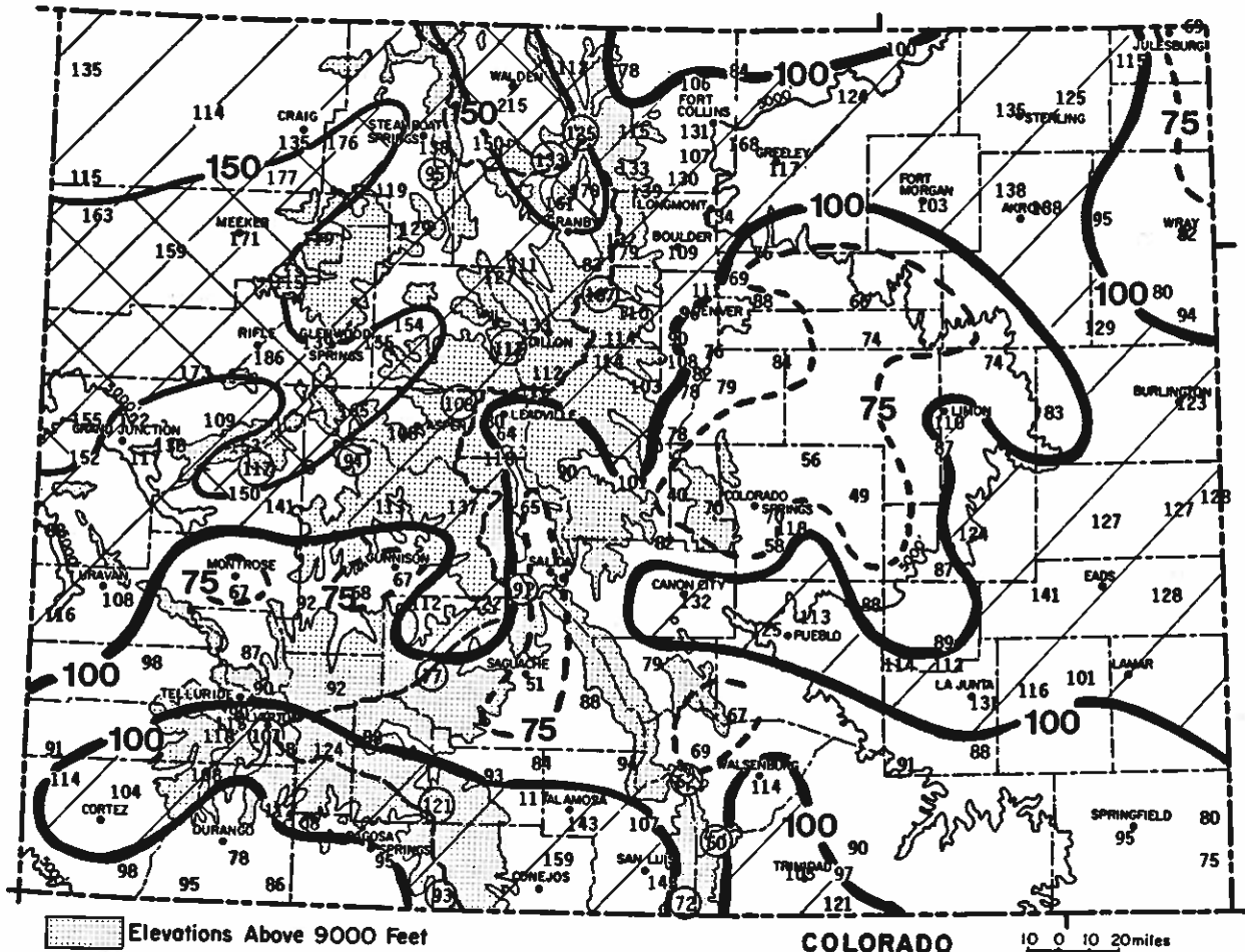
Precipitation for October 1985 through March 1986 as a percent of the 1961-1980 average.
