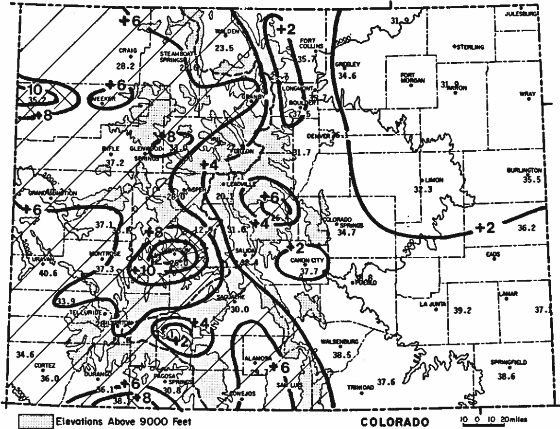
February 1986 temperatures (degrees Fahrenheit) and contours of departures from 1961-1980 averages.
