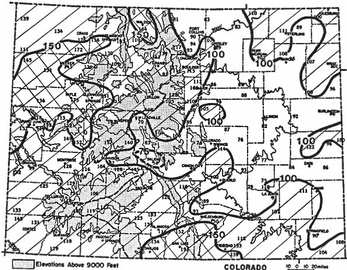
Precipitation for October 1985 through July 1986 as a percent of the 1961-1980 average.
