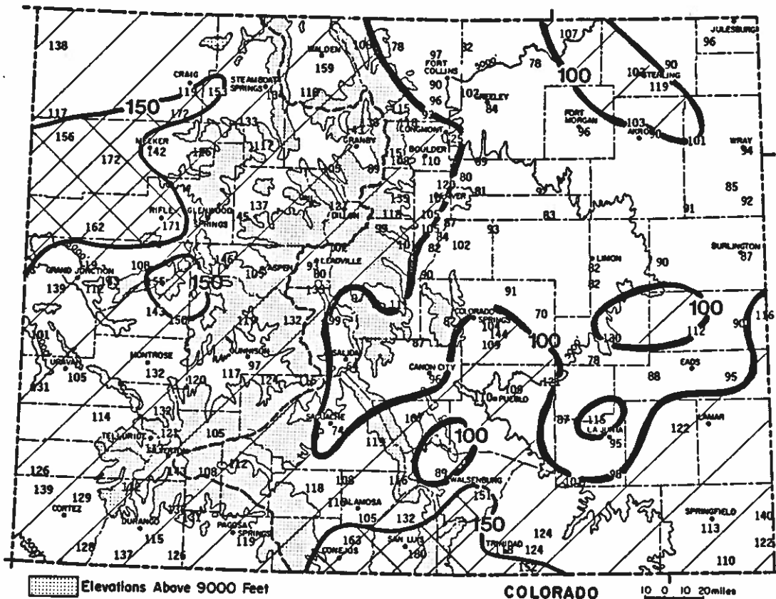
Precipitation for October 1985 through August 1986 as a percent of the 1961-1980 average.
