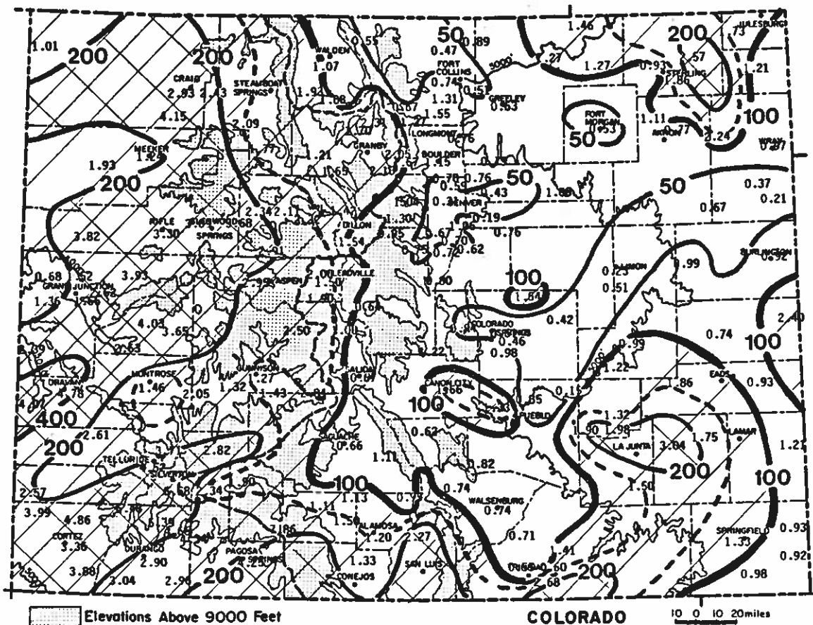
Precipitation amounts (inches) for September 1986 and contours of precipitation as a percent of the 1961-1980 average. The dashed line represents 150% of average.
