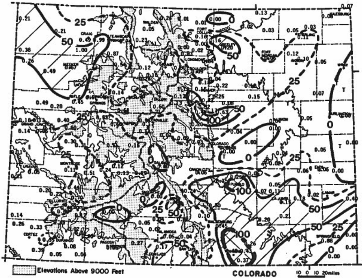
Precipitation amounts (inches) for January 1986 and contours of precipitation as a percent of the 1961-1980 average.
