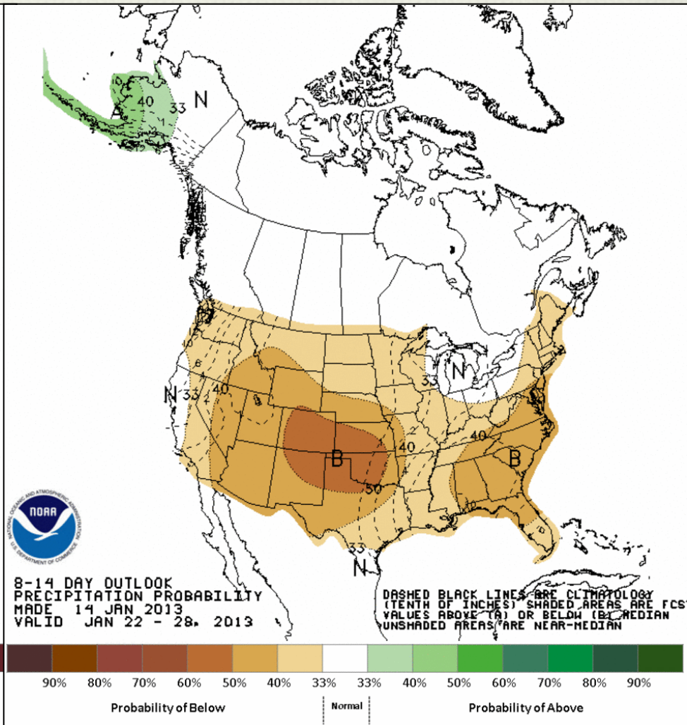
Precipitation Anomalies
