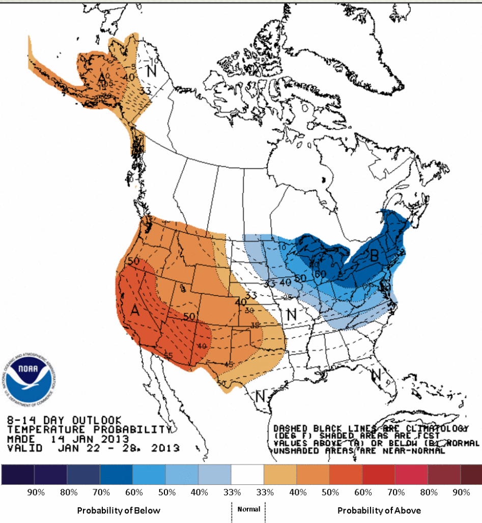
Temperature Anomalies
