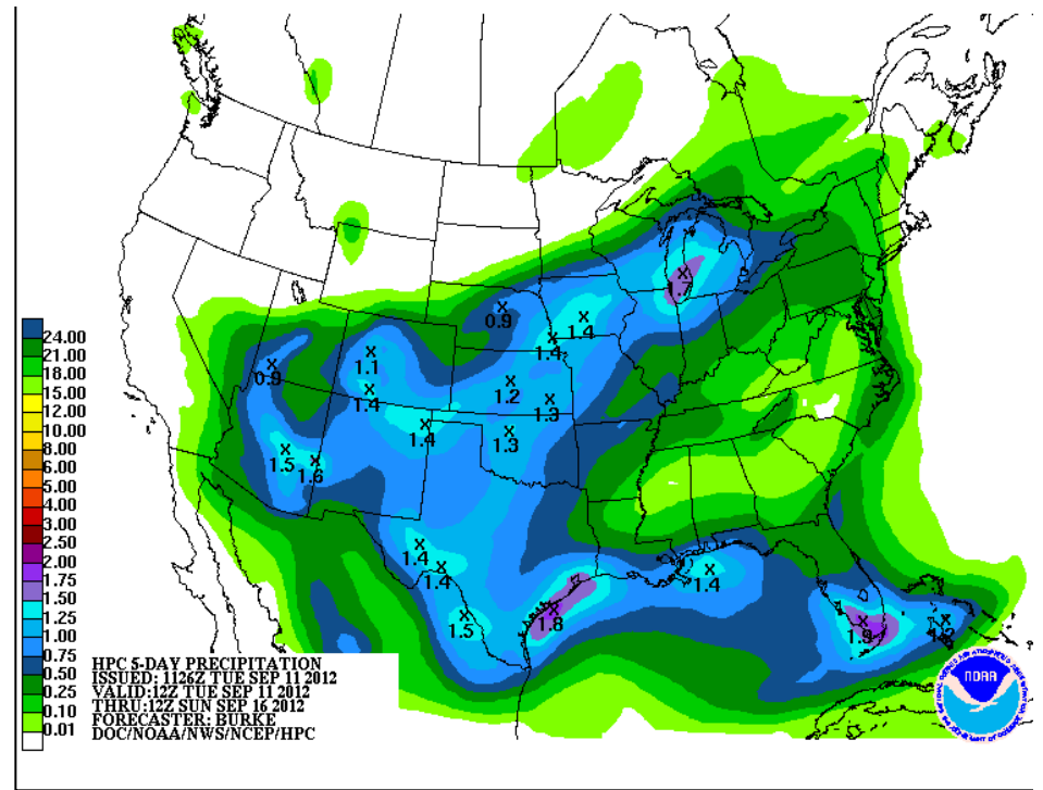
Fig. 6: HPC's quantitative precipitation forecast through 12UTC Sunday.
