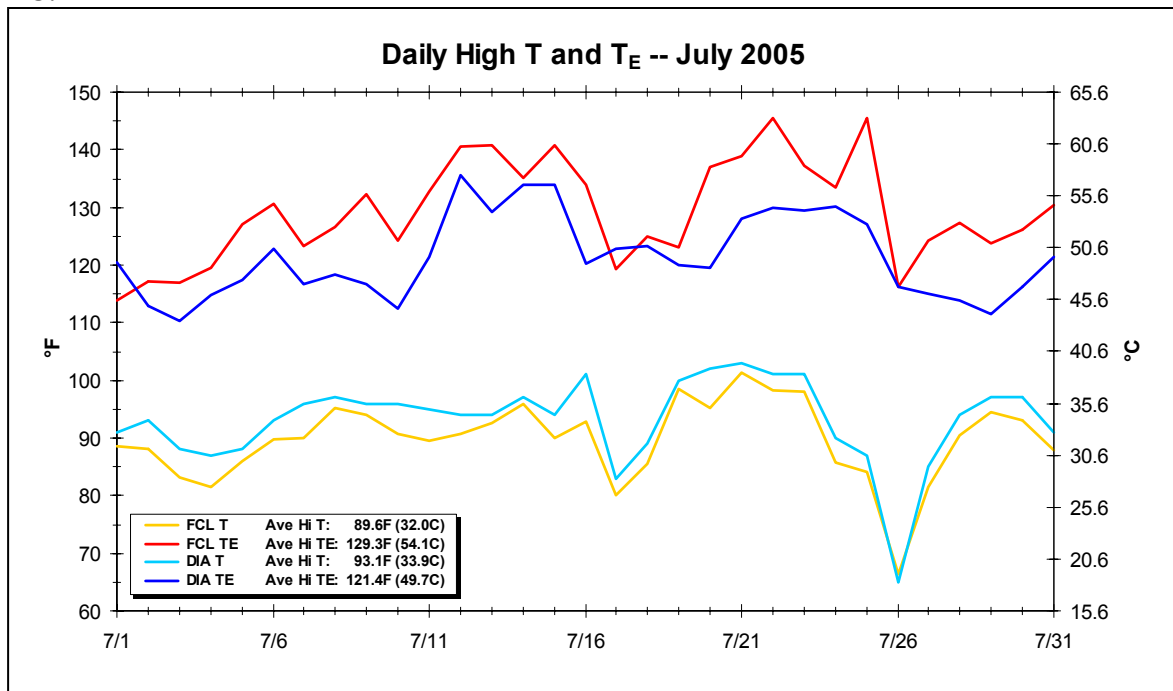
Figure 9. Hourly data from automated weather stations at FCL and DIA are used to pick and calculate the highest air temperature and effective temperature for each day in July 2002 (a), July 2003 (b), and July 2005 (c). In all three months, the average high air temperature is higher at DIA, while the average high effective temperature is higher at FCL.
