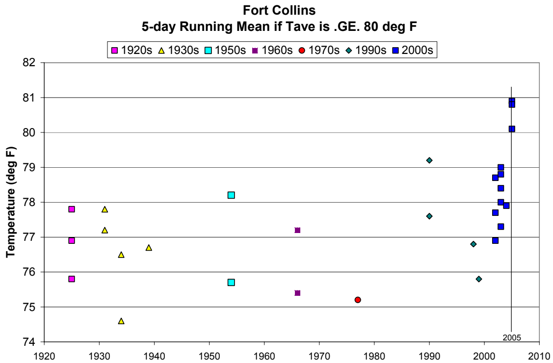
Figure 8. Time series, 1889 – 2005, of 5-day centered mean daily temperatures ( ^{\circ} F) for the Fort Collins, CO weather station for each day with a mean temperature (average of the high and low for the day) of 80^{\circ} F or higher. The threshold of 80^{\circ} F or higher was used because there were no days above 83^{\circ} F.
