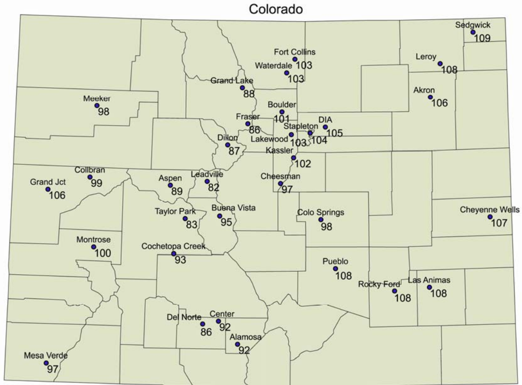
Figure 3. Locations of the weather stations used in this study and their highest recorded daily maximum temperature for July 2005.
