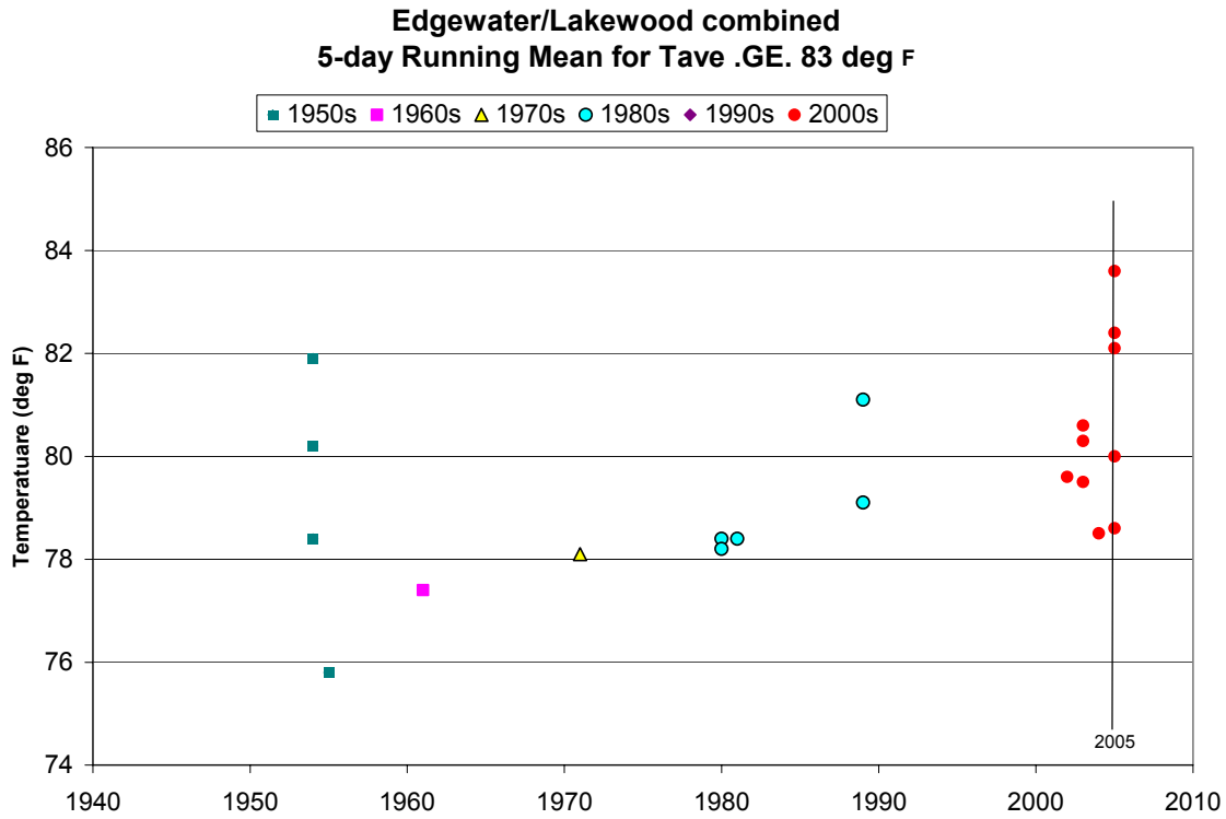
Figure 7. Time series of 5-day centered mean daily temperatures (°F) for each day with a mean temperature (average of the high and low for the day) of 83°F or higher. This time series incorporates data from the Edgewater, CO, cooperative weather station 1948-1962 and the nearby Lakewood, CO, cooperative station from 1962-2005.
